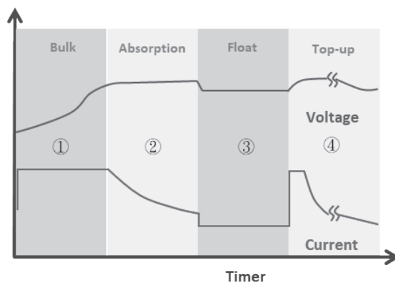
Charge Curve
