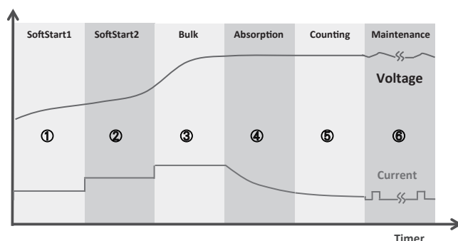
Charging Curve
