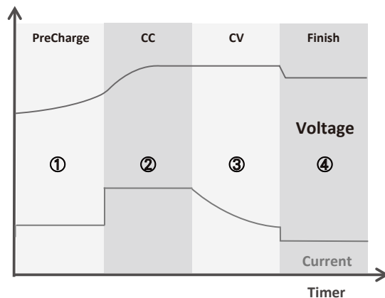
Charge Curve
